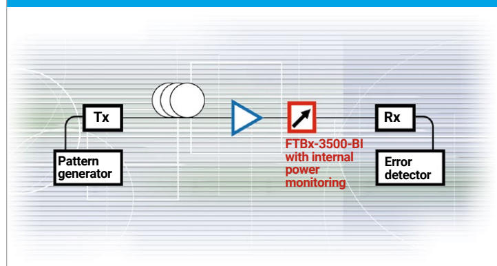
Typical receiver sensitivity setup
