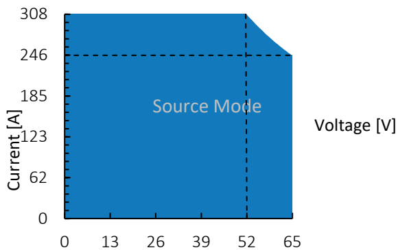
Figure 1: TC.P.16.65.400.S, voltage / current operating area.
