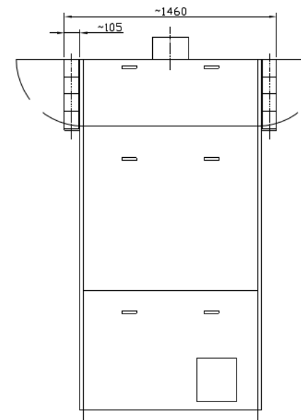
Side view of the Reactor Cabinet/ Glovebox
